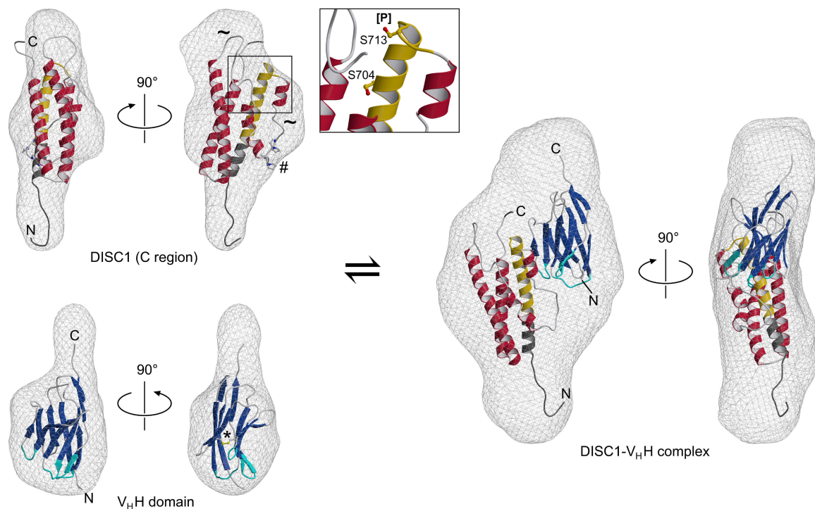
Fig 5. Ab initio SAXS reconstructions and molecular models for the DISC1 691-836 protein, the V H H domain, and their complex. The hypothetical DISC1 model (upper left) features a single domain containing three longer and three shorter \alpha -helices. Similar to the terminal segments, the two extended loops (tilde symbols) are suggested to be poorly ordered. The positions of functionally important residues S704 and S713 are indicated in a close-up view. Also note the proline-rich motif (ball-and-stick representation, marked by a hash), which is predicted to be readily accessible for protein-protein interactions. The 691–715 region, suggested to participate in the epitope for the nanobody, is highlighted in gold while cloning artifacts at the termini are colored dark gray. The model of the V H H antibody (lower left) displays a canonical immunoglobulin fold, including a conserved disulfide bridge (ball-and-stick model, marked by an asterisk). The CDR segments, as defined by the Chothia criteria [60], are highlighted in cyan. Finally, the DISC1 691-836 fragment and the nanobody are predicted to interact in a complex (right) featuring a 1:1 stoichiometry.
